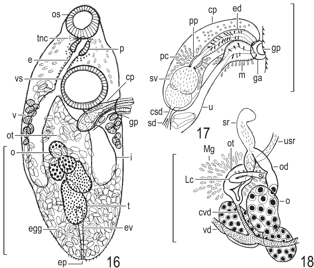
Figs. 16–18. Asymphylostrema monostyloides , adults found in intestine of Cobitis biwae . — 16, holotype (NSMT-PI 3776), entire body, ventral view; 17, paratype (NSMT-PI 3776), terminal genitalia, ventral view; 18, specimen (NSMT-PI 5474), ovarian complex, dorsal view. Scale bars: 0.3 mm in Fig. 16; 0.1 mm in Figs. 17–18.
