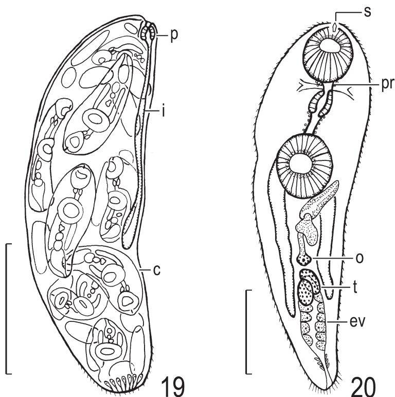
Figs. 19–20. Asymphylostrema monostyloides , life cycle, [daughter (?)] redia (NSMT-PI 5496) and cercaria (MPM Coll. No. 21164) found in Semisulcospira libertina . — 19, redia; 20, cercaria, penetration glands omitted. Scale bars: 0.3 mm in Fig. 19; 0.1 mm in Fig. 20.
