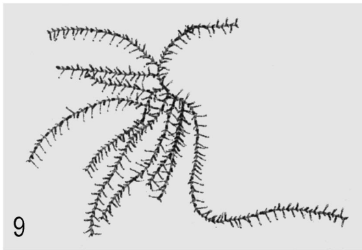
Fig. 9. Asymphylogora innominata , life cycle, photograph of an aggregation of cercariae, scale unknown. Reproduced from Shimazu (2007).
