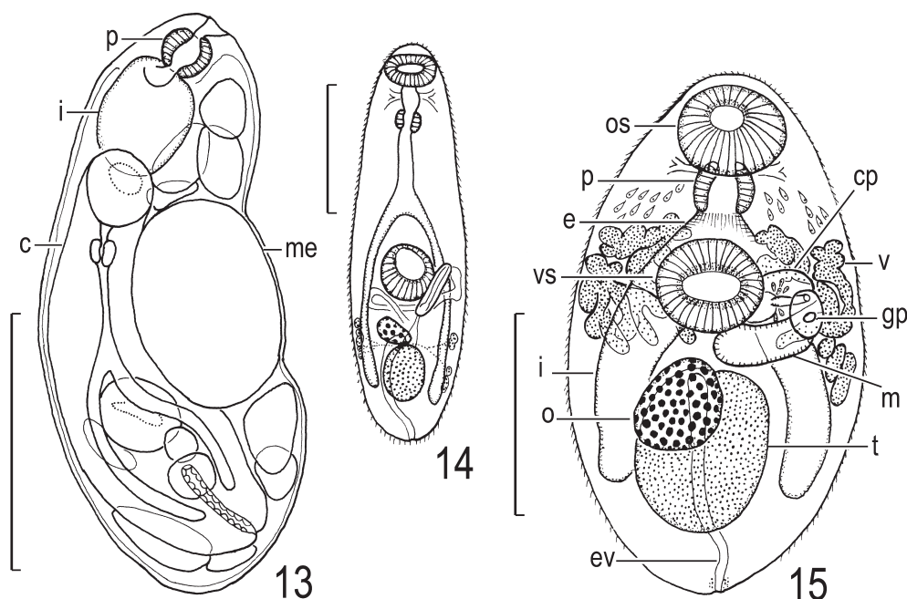
Figs. 13–14. Asymphylogadora japonica , life cycle. — 13, [daughter (?)] redia (MPM Coll. No. 22744) found in Parafossarulus manchouricus japonicus ; 14, excysted metacercaria (MPM Coll. No. 22281) found in Pa. manchouricus japonicus , ventral view. Scale bars: 0.3 mm in Figs. 13–14.
