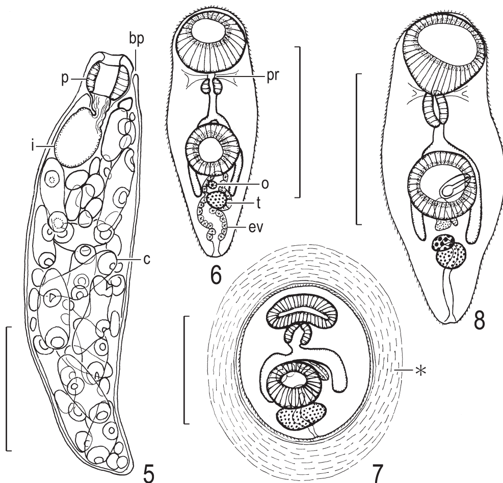
Figs. 5–8. Asymphyiodora innominata , life cycle. — 5, daughter (?) redia (NSMT-PI 5347) found in Semisulcospira libertina ; 6, cercaria (NSMT-PI 5345), ventral view; 7, encysted metacercaria (NSMT-PI 5352) found in connective tissue of mucous membrane of gill raker of Pseudorasbora parva , 16 days after experimental infection, surrounded by tissue of host origin (*); 8, excysted metacercaria (NSMT-PI 5349), 14 days after experimental infection. Scale bars: 0.5 mm in Fig. 5; 0.2 mm in Figs. 6–8.
