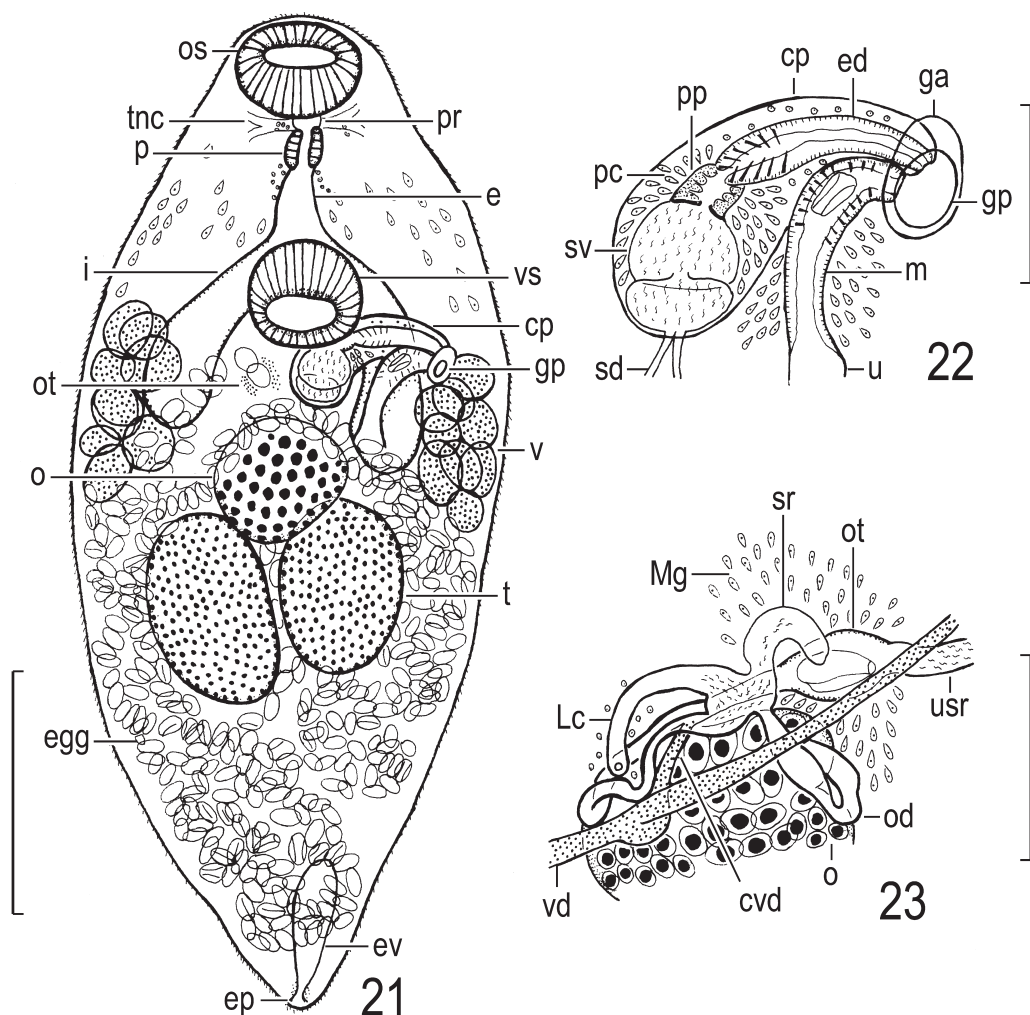
Figs. 21–23. Palaeorchis diplorchis , adults found in intestine of Pseudogobio esocinus esocinus . — 21, holotype (MPM Coll. No. 22273), entire body, ventral view; 22, holotype, terminal genitalia, ventral view; 23, specimen (NSMT-PI 3980), ovarian complex, dorsal view. Scale bars: 0.3 mm in Fig. 21; 0.1 mm in Figs. 22–23.
