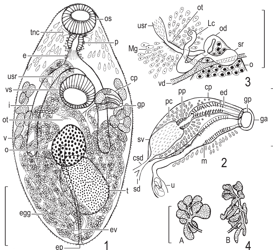
Figs. 1–4. Asymphylodora innominata , adult specimens. — 1, specimen (NSMT-PI 3692) found in intestine of Tribolodon hakonensis , entire body, ventral view; 2, specimen (NSMT-PI 5334) found in intestine of T. hakonensis , terminal genitalia, ventral view; 3, specimen (NSMT-PI 5334), ovarian complex, dorsal view; 4, specimens (NSMT-PI 3685) found in intestine of Opsariichthys uncirostris uncirostris , vitelline follicles in young adult specimen (A) and old adult specimen (B), ventral view. Fig. 4 redrawn from Shimazu et al. (2011). Scale bars: 0.3 mm in Figs. 1 and 4; 0.1 mm in Figs. 2–3.
