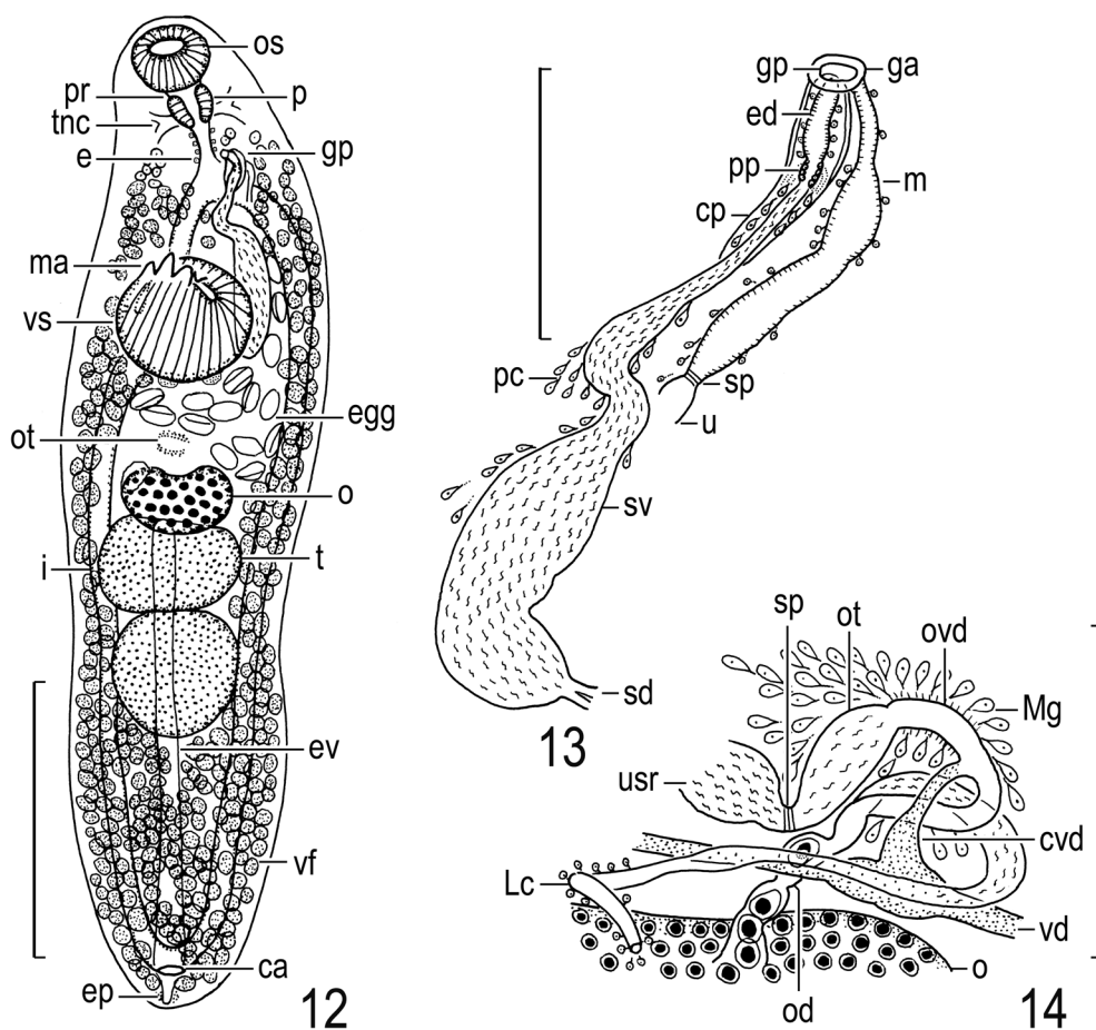
Figs. 12–14. Opecoelus ukigori , adult specimens found in intestine of Gymnogobius opperiens . 12, holotype (NSMT-PI 3114), entire body, ventral view; 13, paratype (NSMT-PI 3116), terminal genitalia, ventral view; 14, paratype (NSMT-PI 3116), ovarian complex, dorsal view. Scale bars: 0.5 mm in Fig. 12; 0.2 mm in Figs. 13–14.
