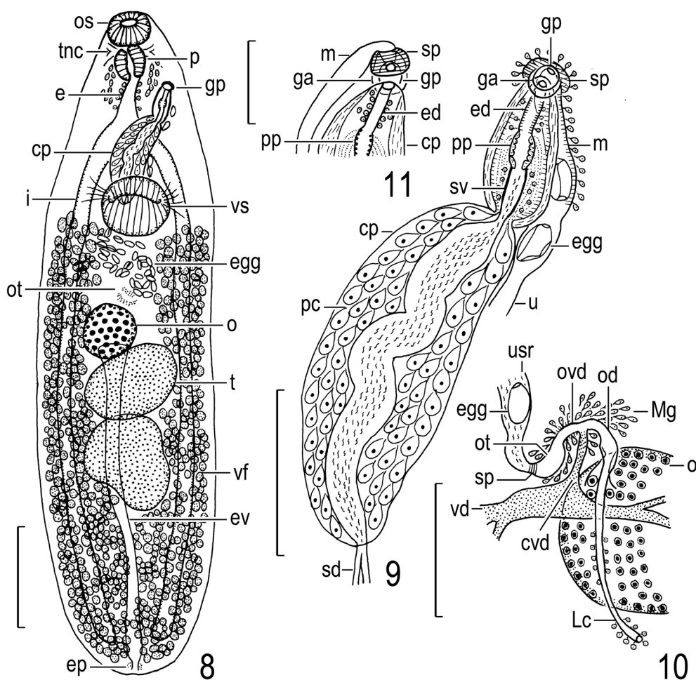
Figs. 8–10. Dimerosaccus oncorhynchi , neotype, adult specimen (NSMT-PI 5850) found in intestine of Oncorhynchus masou ishikawae . 8, entire body, ventral view; 9, terminal genitalia, ventral view; 10, ovarian complex, dorsal view. Scale bars: 0.5 mm in Fig. 8; 0.2 mm in Figs. 9–10.
