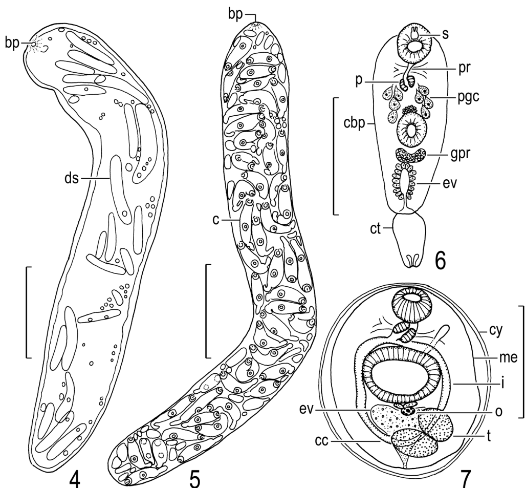
Figs. 4–7. Coitocaecum plagiorchis (continued), life cycle. 4, mother sporocyst found in Semisulcospira libertina , site of infection not given; 5, daughter sporocyst (NSMT-PI 5439) found in S. reiniana , site of infection perhaps rectum; 6, cercaria (NSMT-PI 5442) found in S. libertina , ventral view; 7, encysted metacercaria (NSMT-PI 5443) found in Neocardina denticulata , 24–25 days after experimental infection, site of infection not given, ventral view. Scale bars: 0.5 mm in Figs. 4–5; 0.2 mm in Fig. 7; 0.1 mm in Fig. 6.
