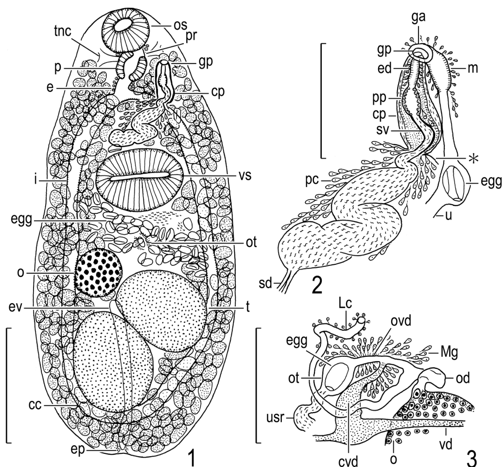
Figs. 1–3. Coitocaecum plagiorchis , adult specimen (NSMT-PI 5527) found in intestine of Tridentiger brevispinis . 1, entire body, ventral view; 2, terminal genitalia, remnant (*) of ruptured posterior portion of cirrus pouch, ventral view; 3, ovarian complex, dorsal view. Scale bars: 0.5 mm in Fig. 1; 0.2 mm in Figs. 2–3.
