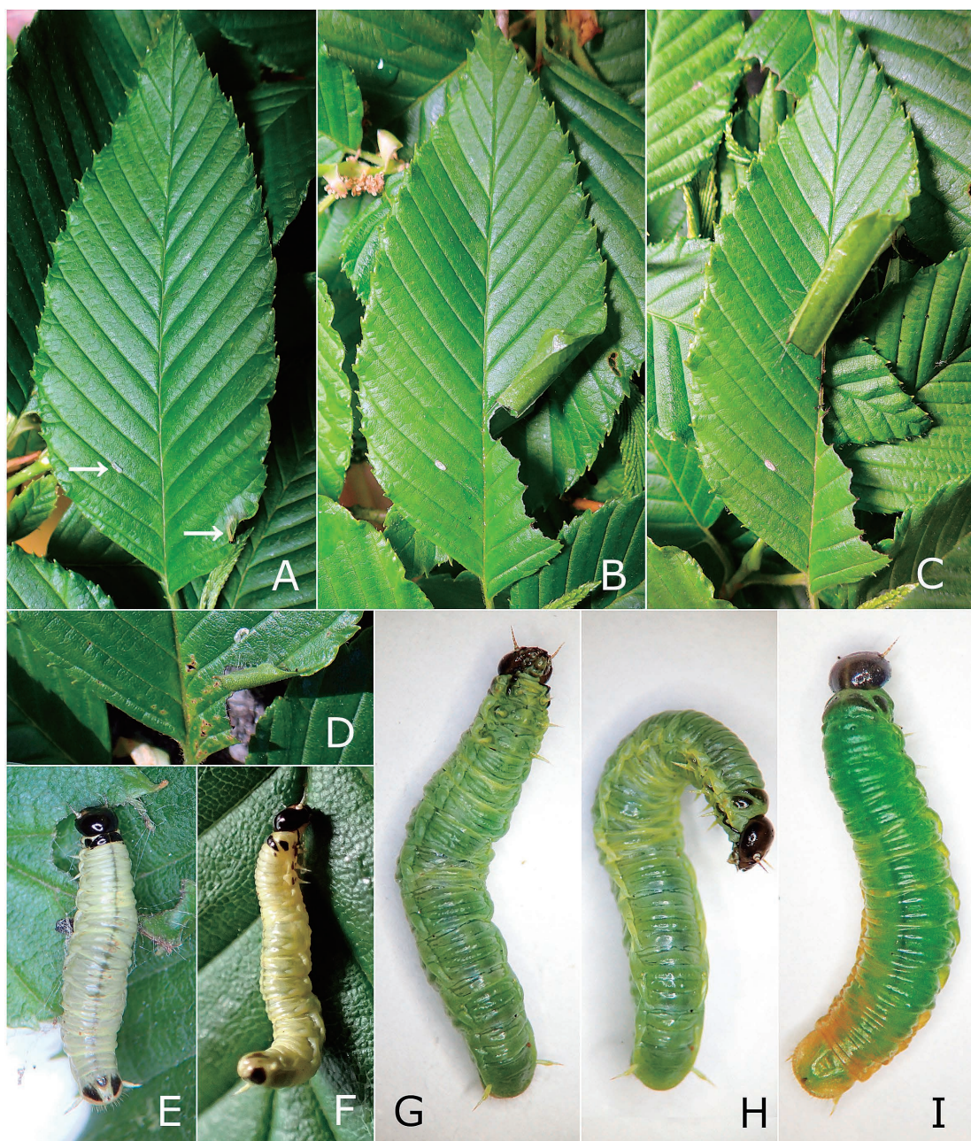
Fig. 1. Pamphilius confusus . A, Leaf of Alnus firma with remains of egg shell (left arrow) and very small larva beginning to make a leaf-roll (right arrow), May 6; B, same leaf with a leaf-roll, May 10; C, same leaf with a large leaf-roll, May 12; D, another leaf with remains of egg shell and a small leaf-roll, May 12; E, middle instar larva, May 18; F, another middle instar larva, May 17; G, H, last instar larva, May 18; I, mature larva, May 18. Photographed by A. Shinohara.
