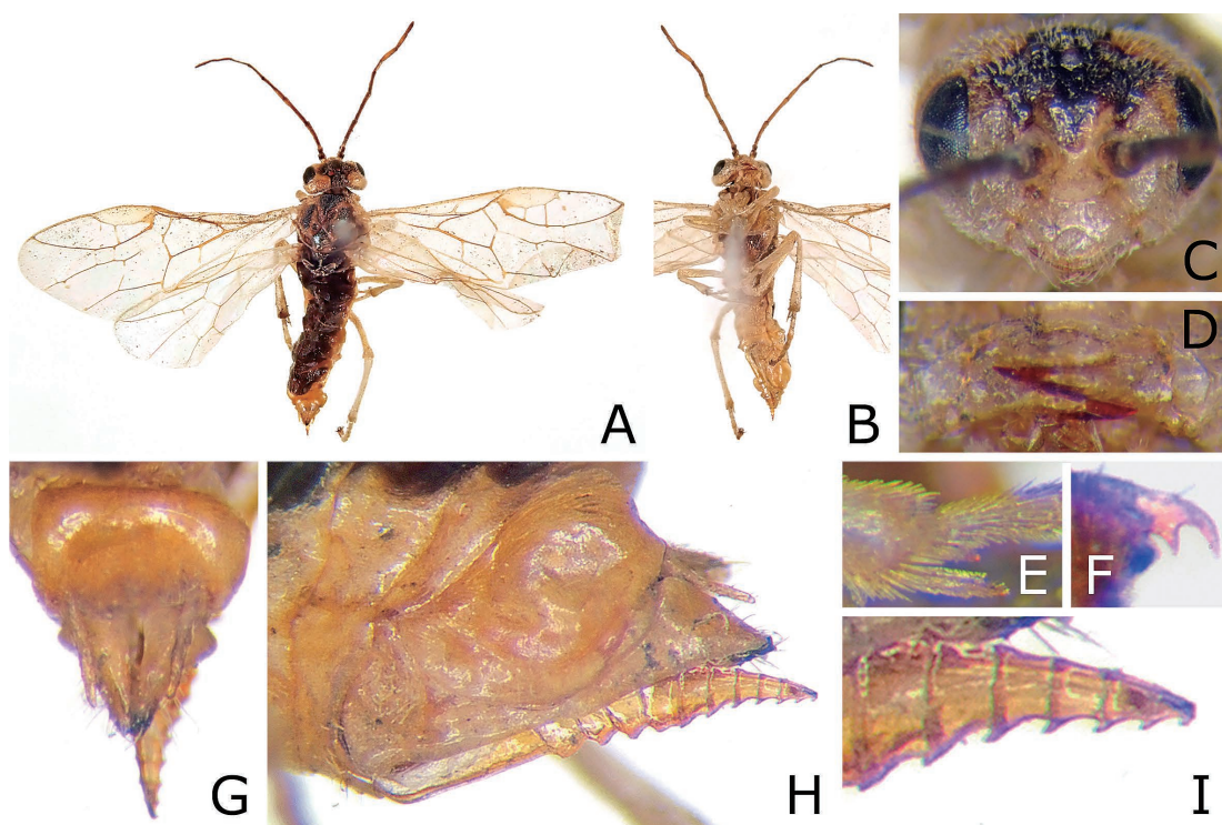
Fig. 2. Nematus cuneiformis , holotype, female. A, B, Dorsal and ventral views; C, head, anterior view; D, mandibles, ventral view (above anterior); E, inner apical fore tibial spur; F, tarsal claw; G, H, apex of abdomen, dorsal and lateral views; I, apex of lancet.
