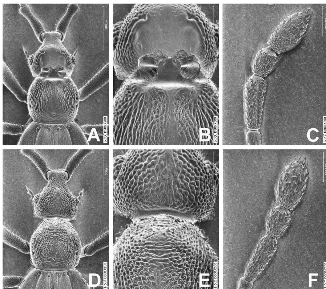
Fig. 6. SEM photos of Nomurais piaoacus Yin et Li. A–C. male; D–F. female. A, D. Head and pronotum in dorsal view; B, E. Ditto, enlarged; C, F. antennal club.
