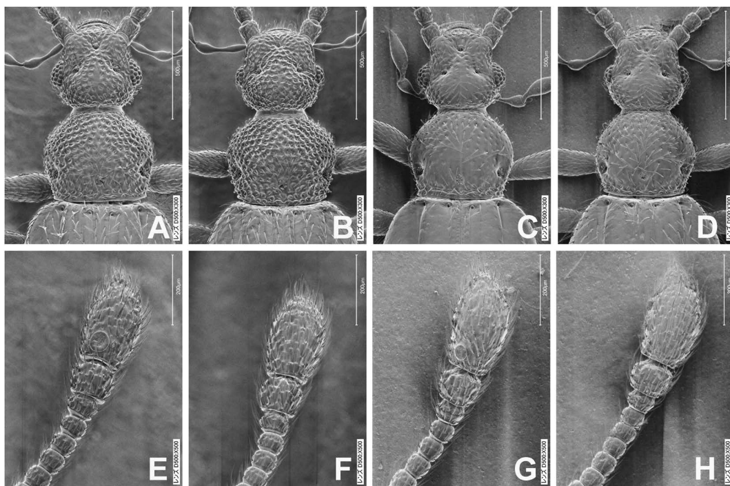
Fig. 5. SEM photos of Triomiscrus spp. A, E. T. vietus Löbl et al. from Mt. Tam Dao, male; B, F. ditto, female; C, G. T. sp. 1 from Mt. Phia Oac, male; D, H. ditto, female. A–D. head and pronotum in dorsal view; E–H. apical segments of antenna.
