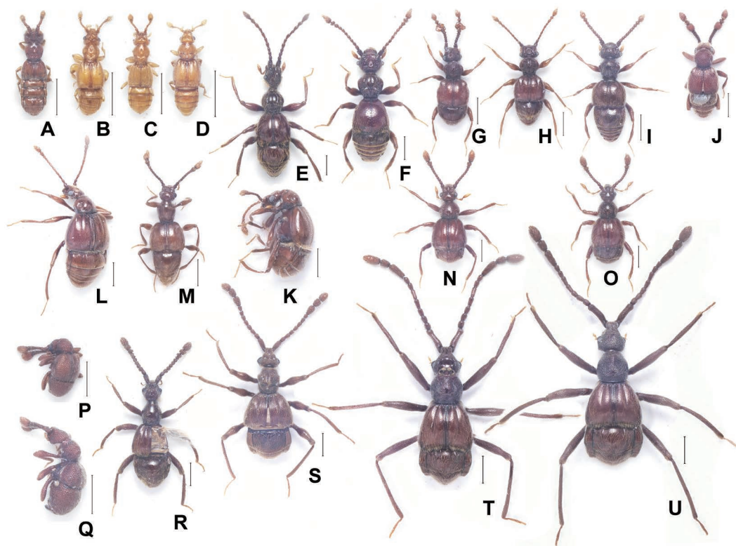
Fig. 3. Photos of pselaphine species collected in the survey. A. Pyxidicerina, gen. and sp. undet 1; B. Pseudoplectus ? sp. 1, male; C. ditto, female; D. Trimium ? sp. 1; E. Intestinarius sp. 1; F. I. sp. 2; G. Trisinus sp. 1; H. T. sp. 2; I. T. sp. 3; J. Sathytes sp. 1; K. Reichenbachia sp. 1; L. Trissemus sp. 1; M. Batraxis sp. 1; N. Triomicrosus sp. 1, male; O. ditto, female; P. Plagiophorus sp. 1; Q. P. sp. 2; R. Pseudophanias sp. 1; S. Pselaphodes sp. 1; T. Nomuraius piaocacus Yin et Lee, 2013, male; U. ditto, female.
